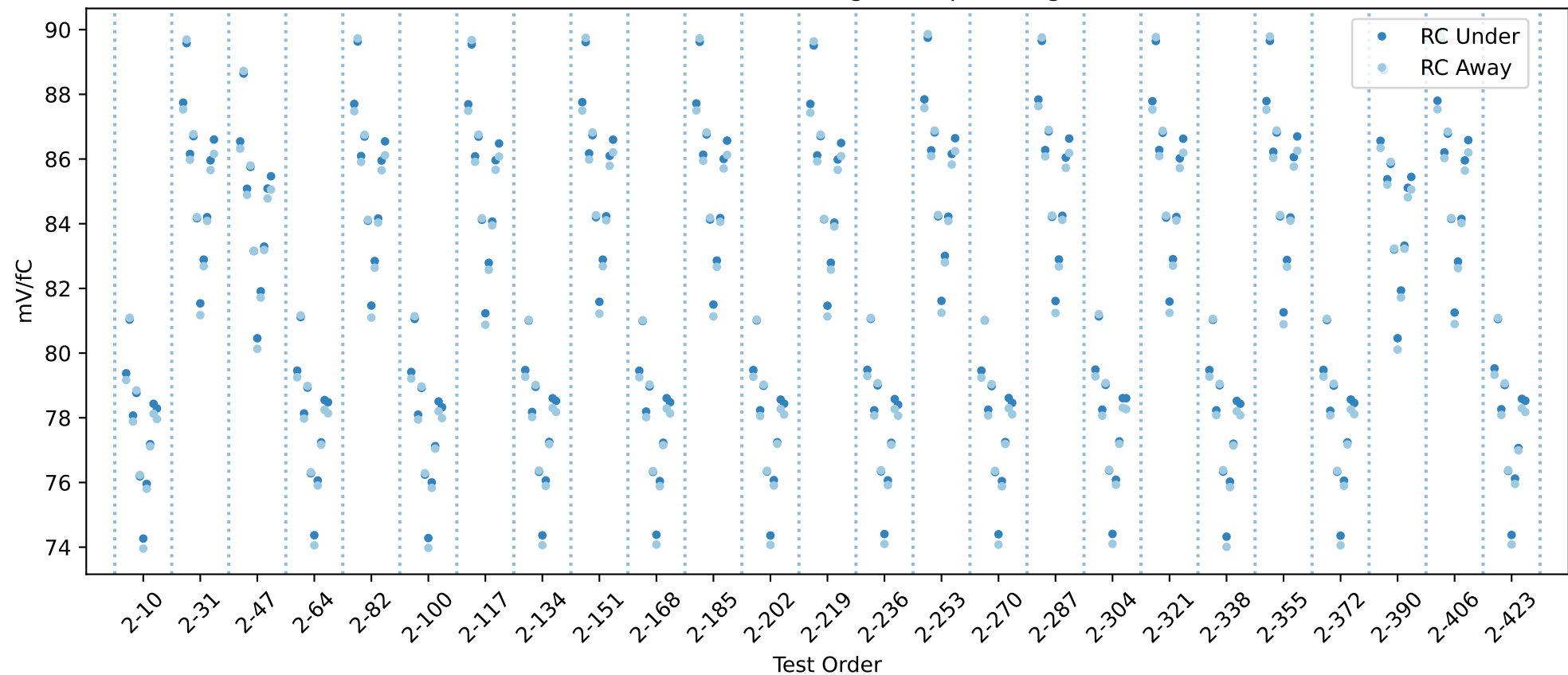
20USBHX2002539 RC gain chip averages
