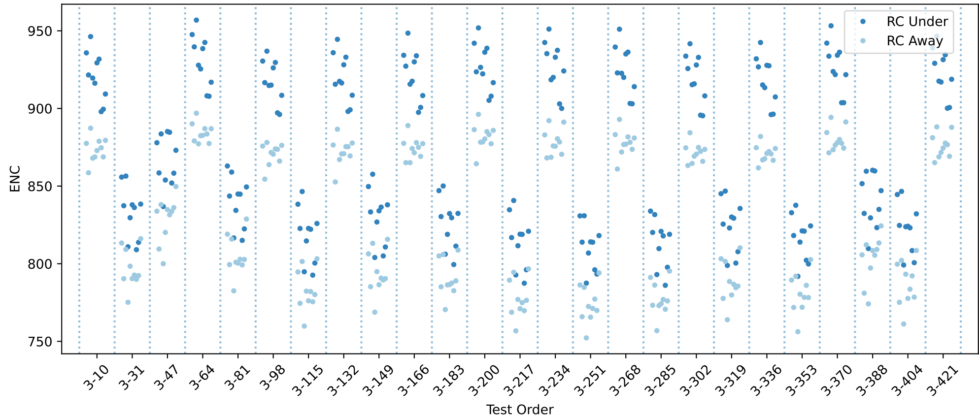
20USBHX2002616 RC innse chip averages
