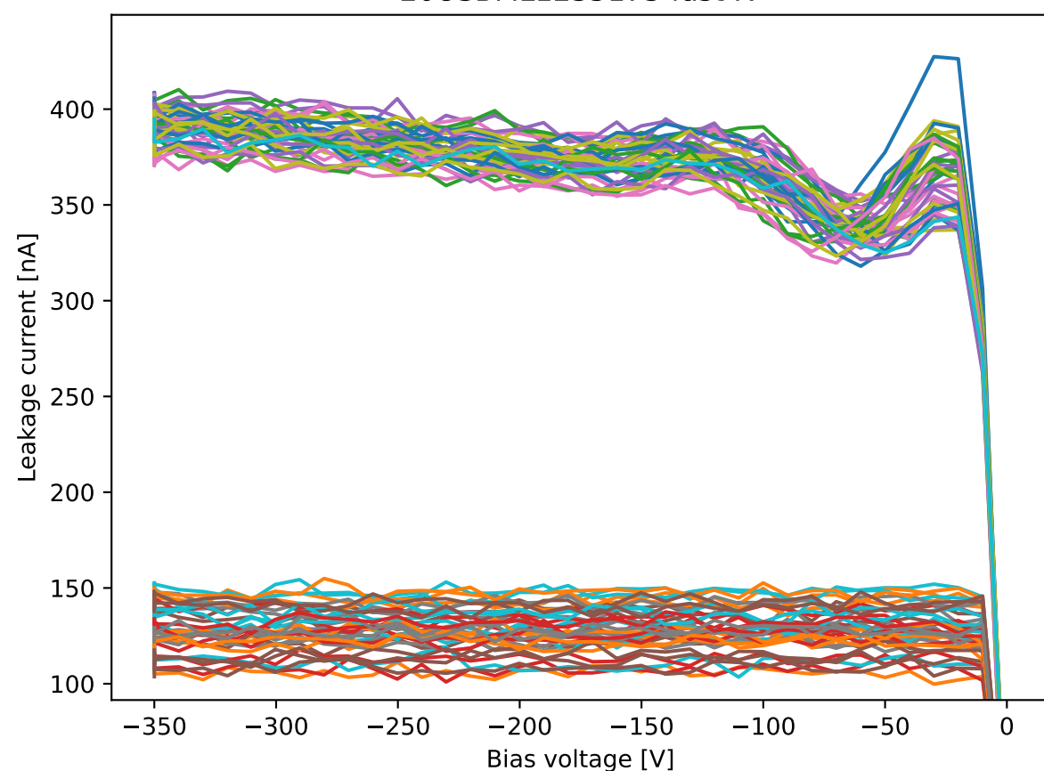
20USBML1235173 fast IV
