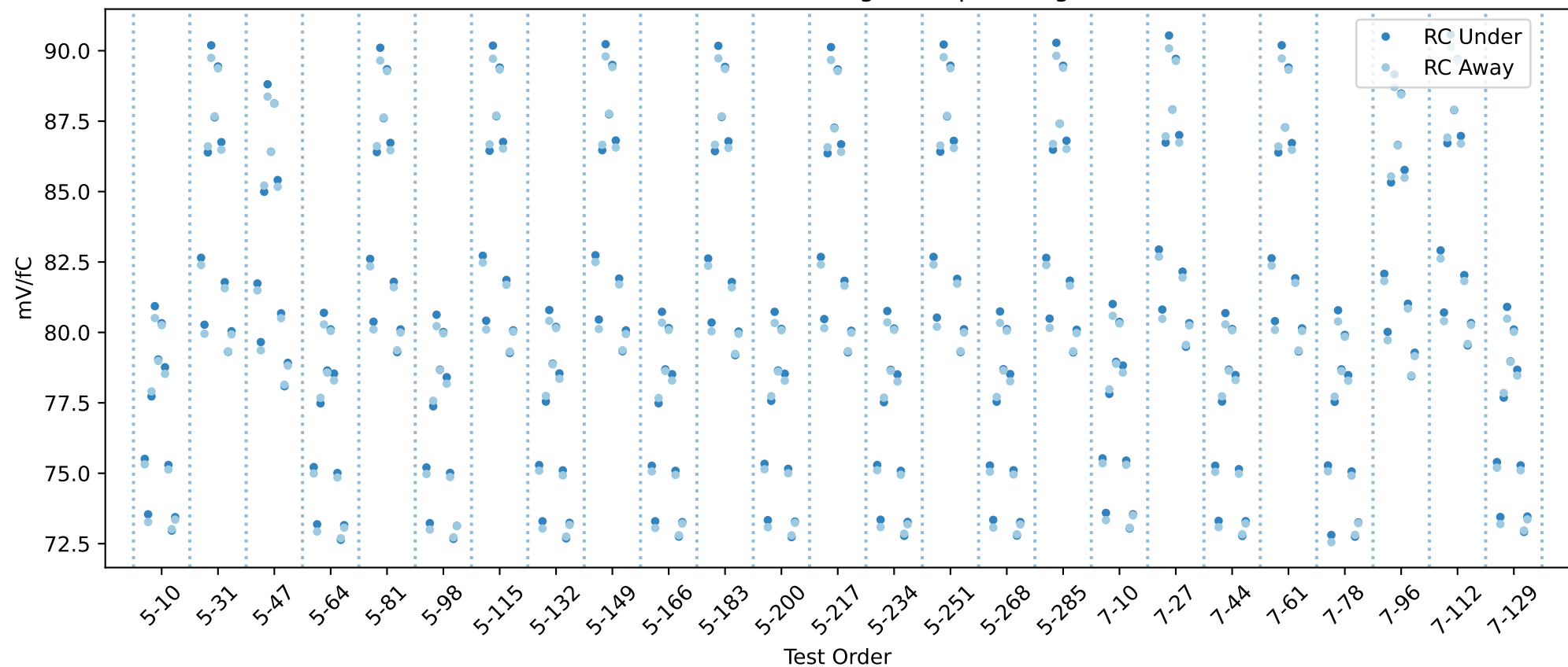
20USBHX2002618 RC gain chip averages
