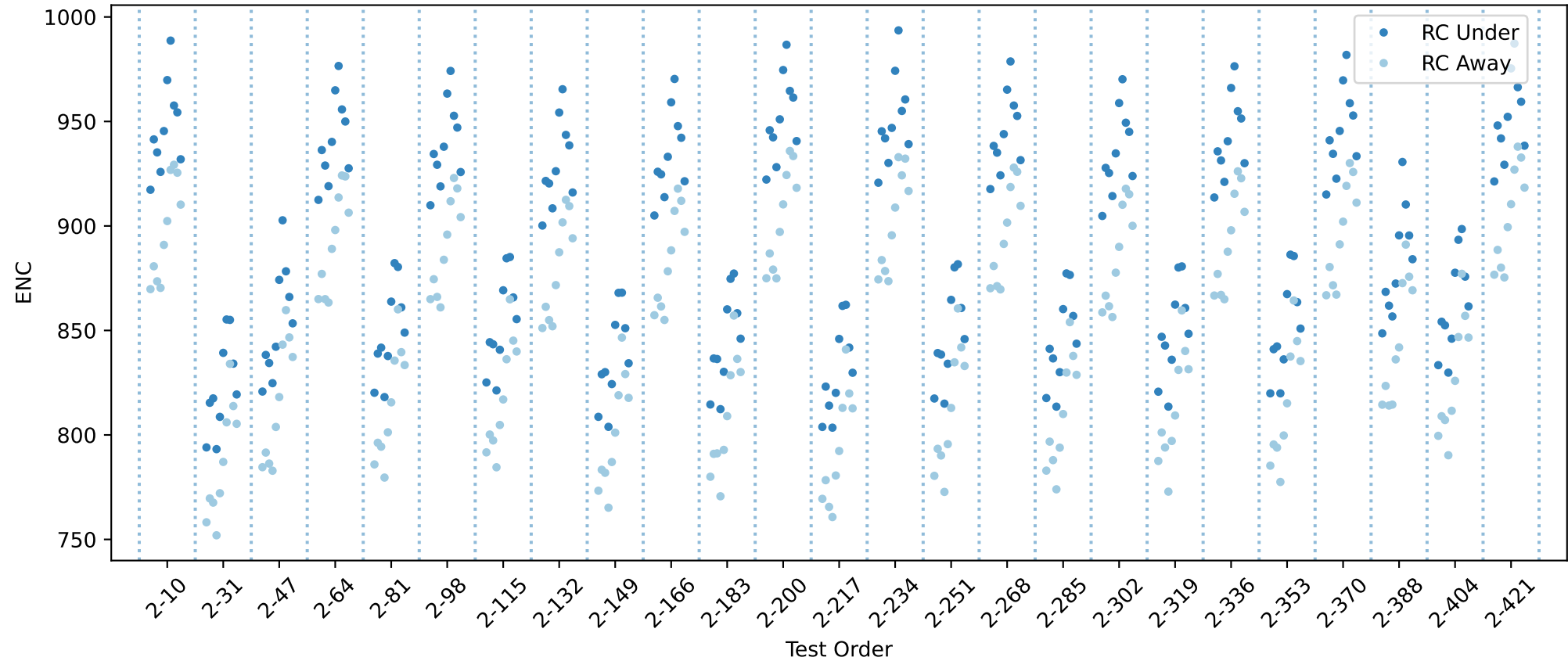
20USBHX2002608 RC innse chip averages
