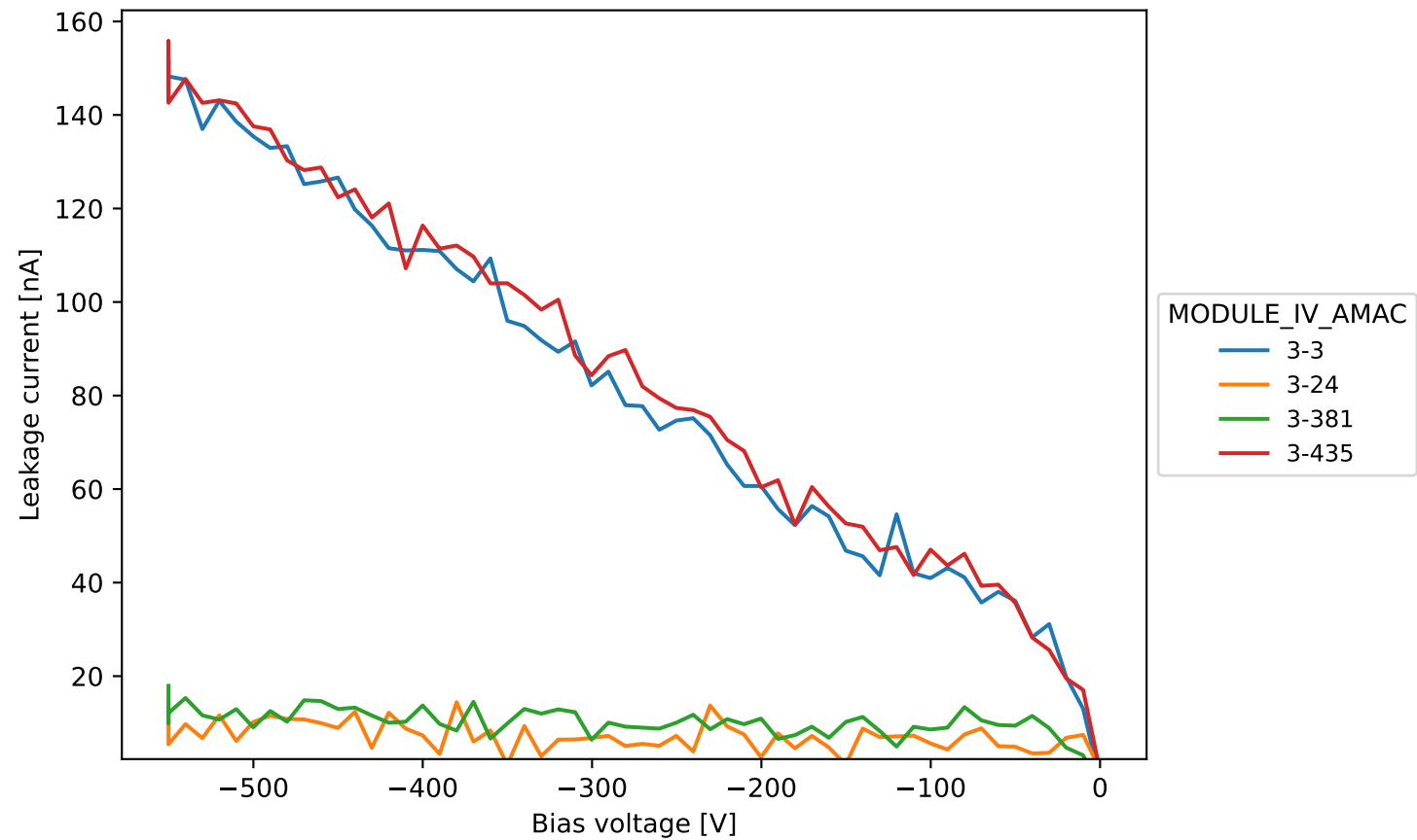
20USBML1235813 standard IV
