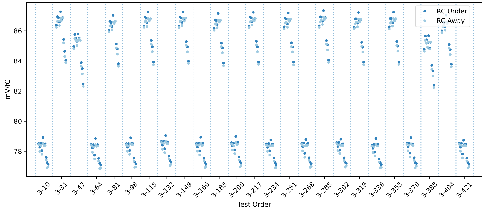
20USBHX2002624 RC gain chip averages
