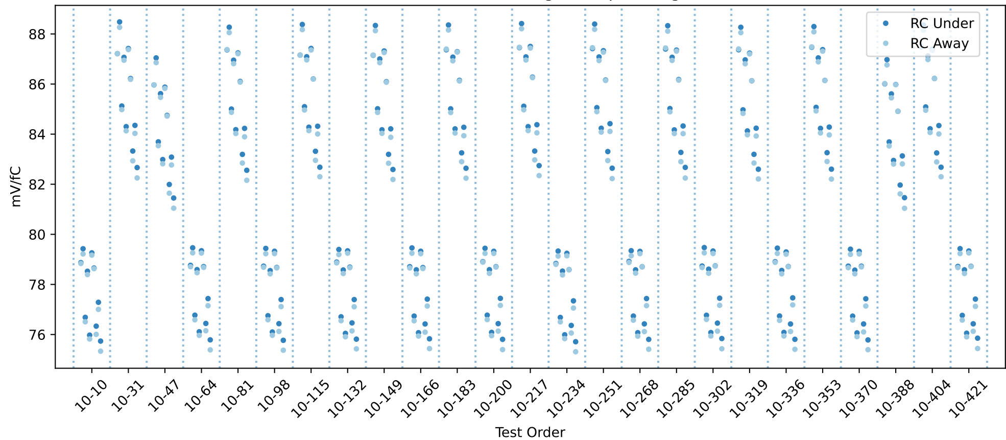
20USBHX2002609 RC gain chip averages
