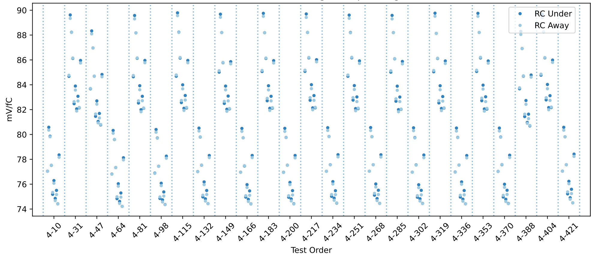
20USBHX2002625 RC gain chip averages
