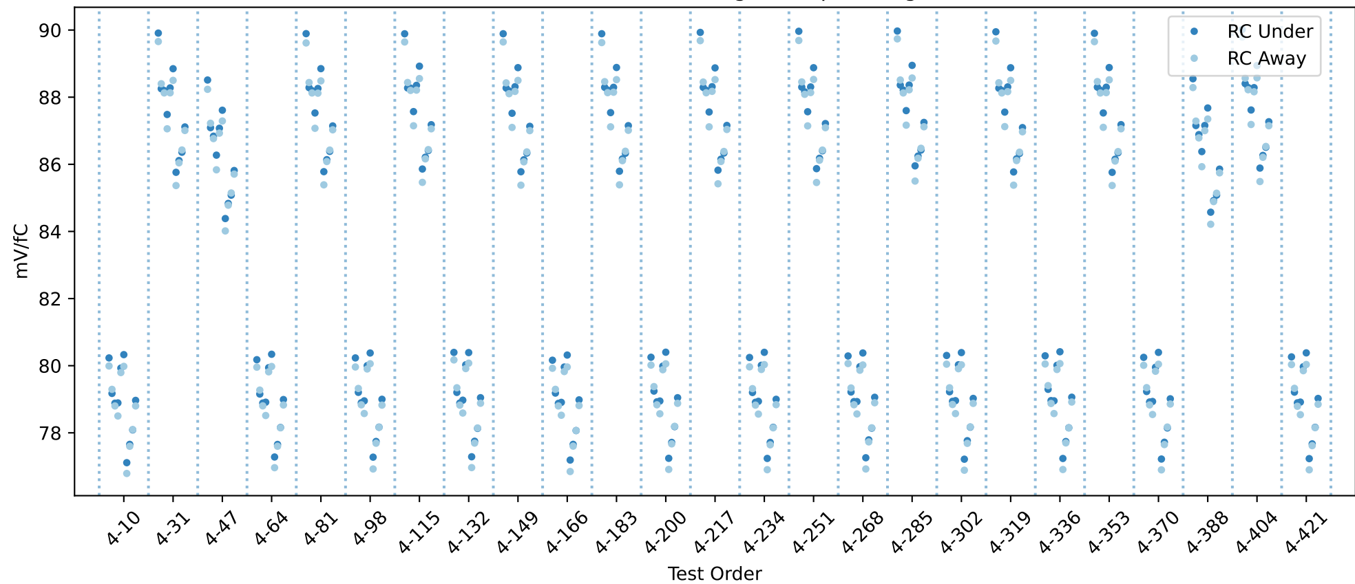
20USBHX2002660 RC gain chip averages
