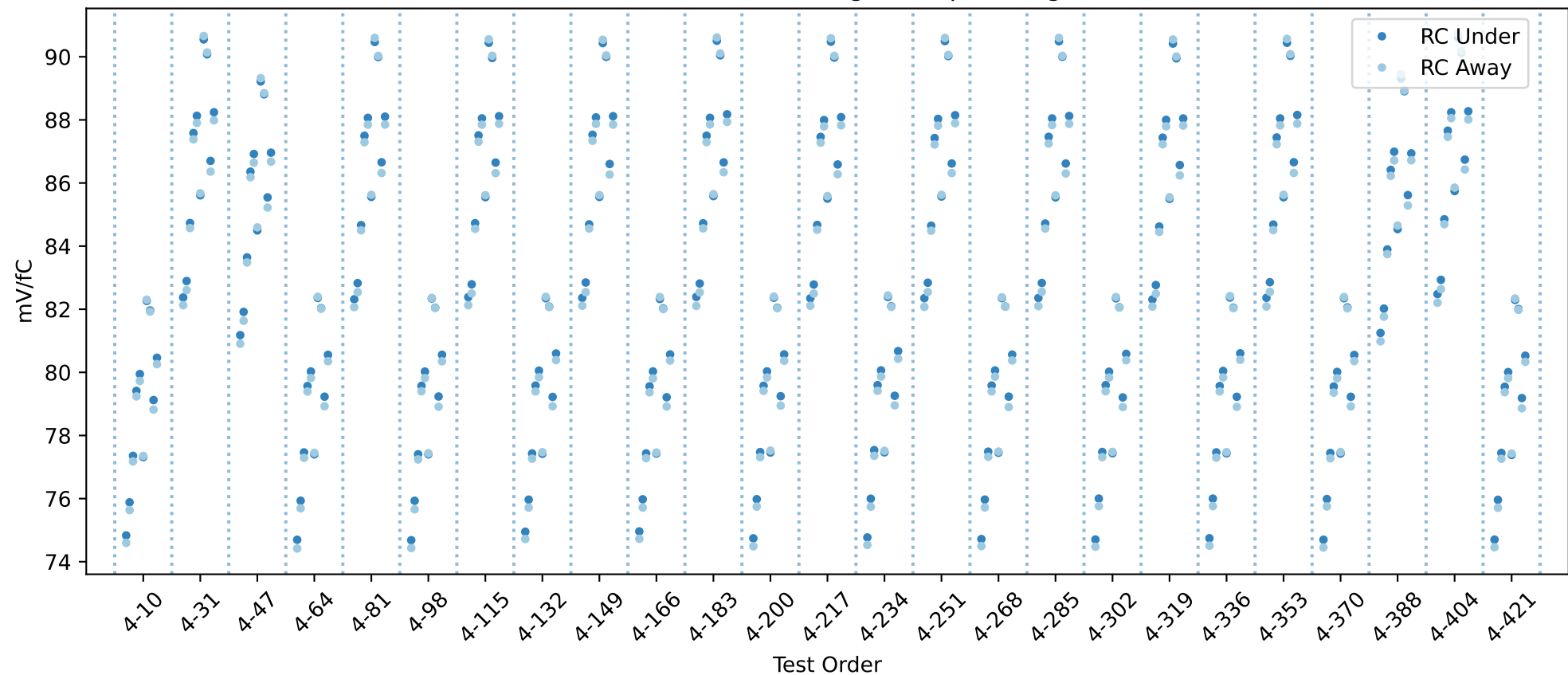
20USBHX2002662 RC gain chip averages
