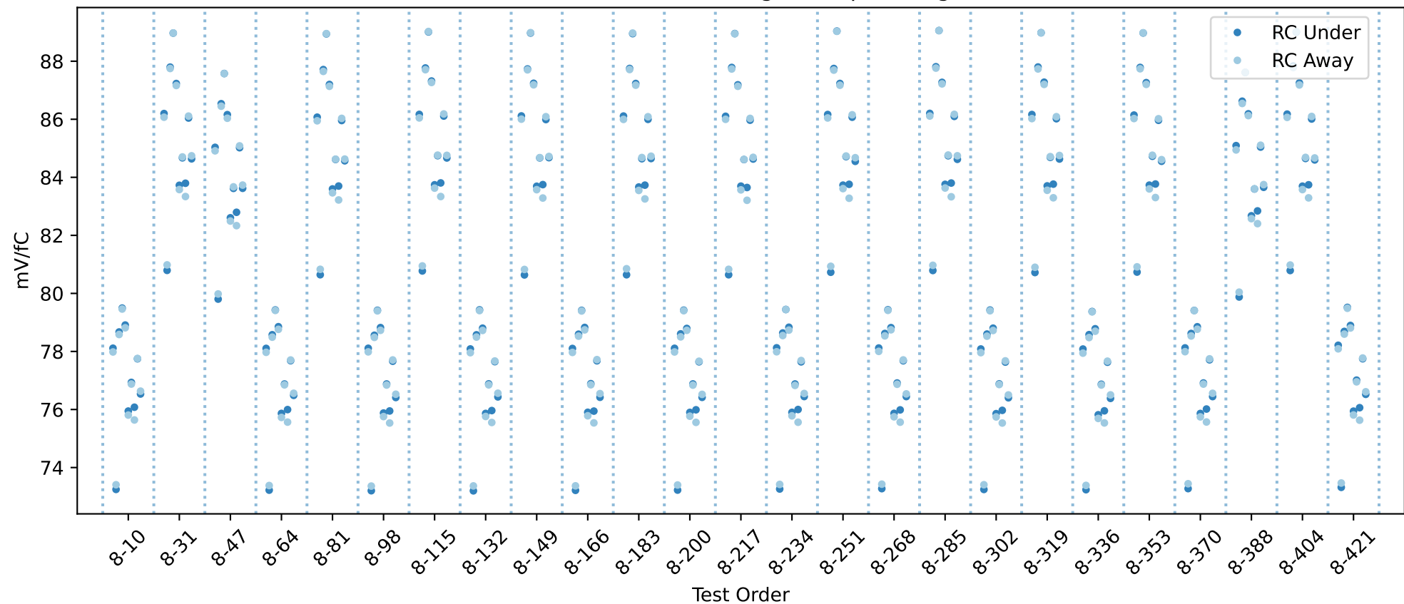
20USBHX2002663 RC gain chip averages
