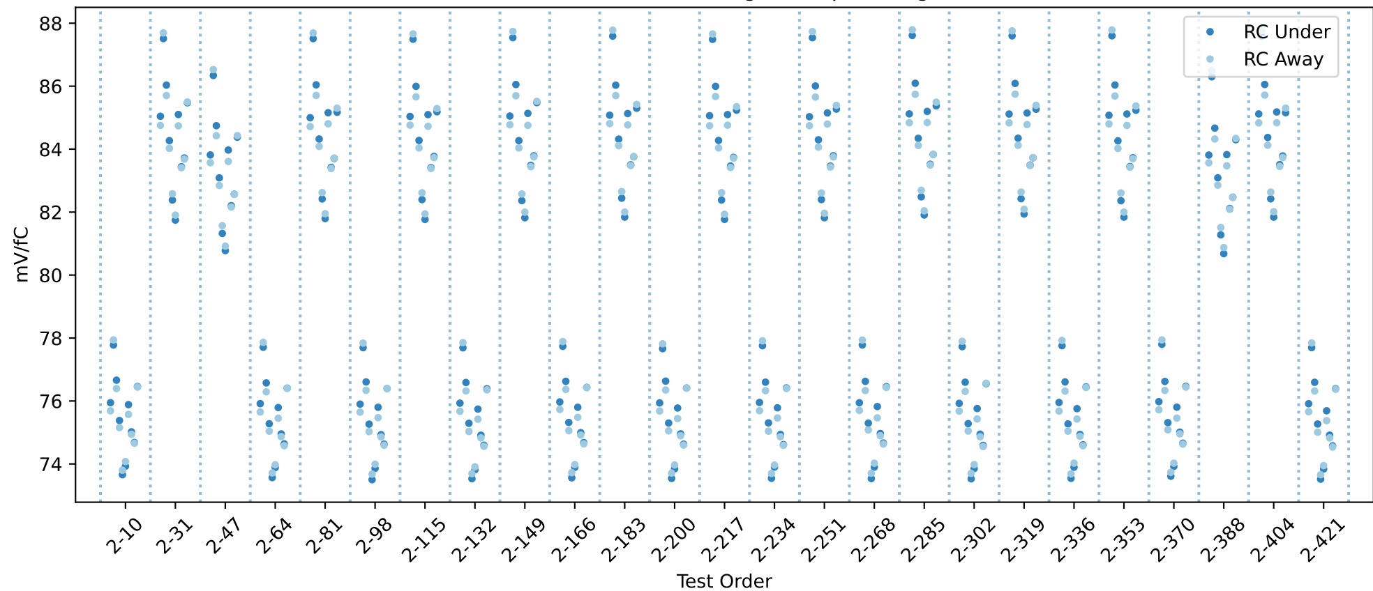
20USBHX2002762 RC gain chip averages
