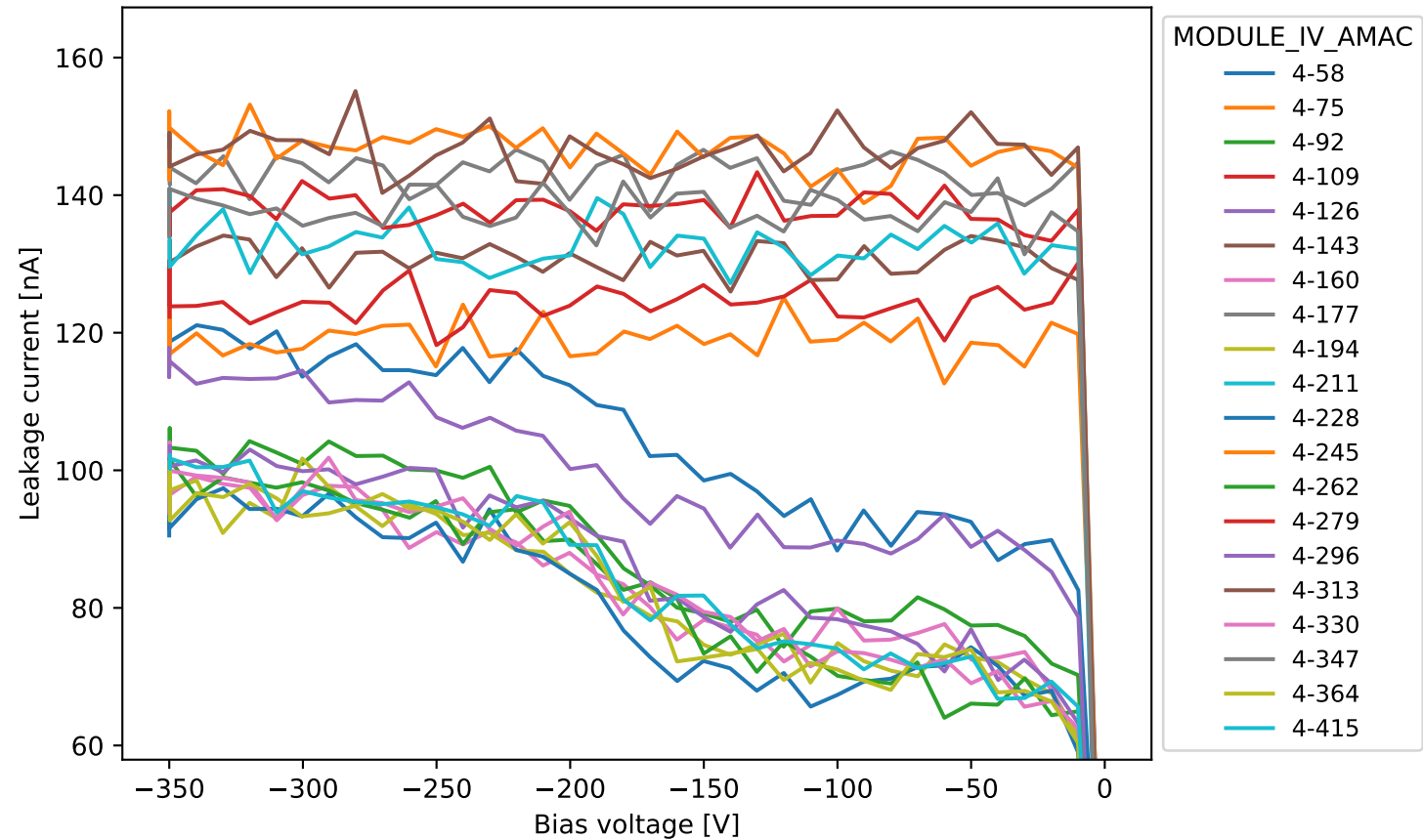
20USBML1236005 fast IV
