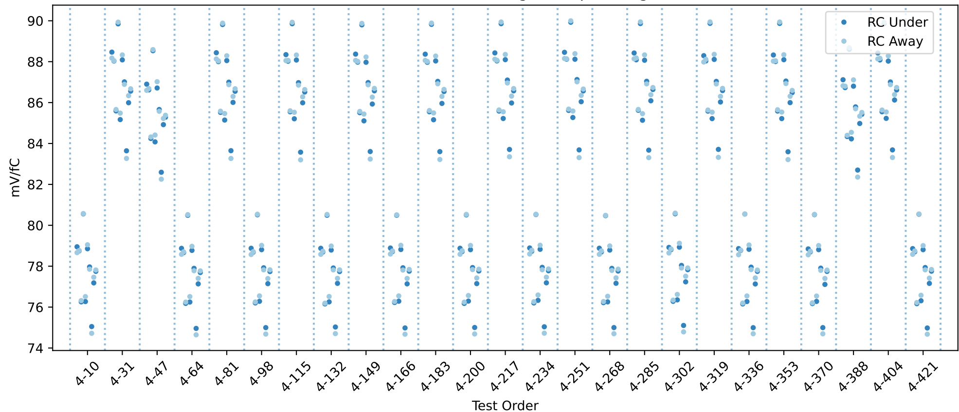
20USBHX2002757 RC gain chip averages
