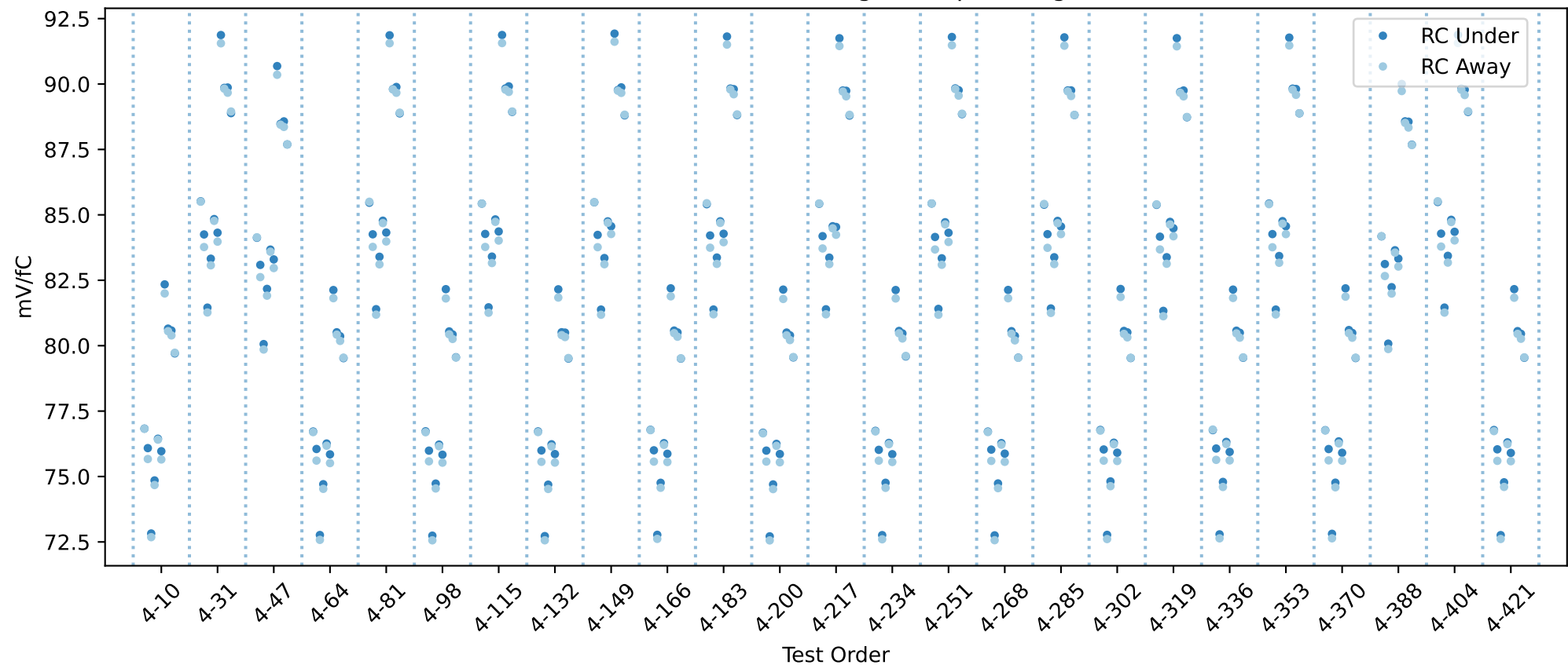
20USBHX2002767 RC gain chip averages
