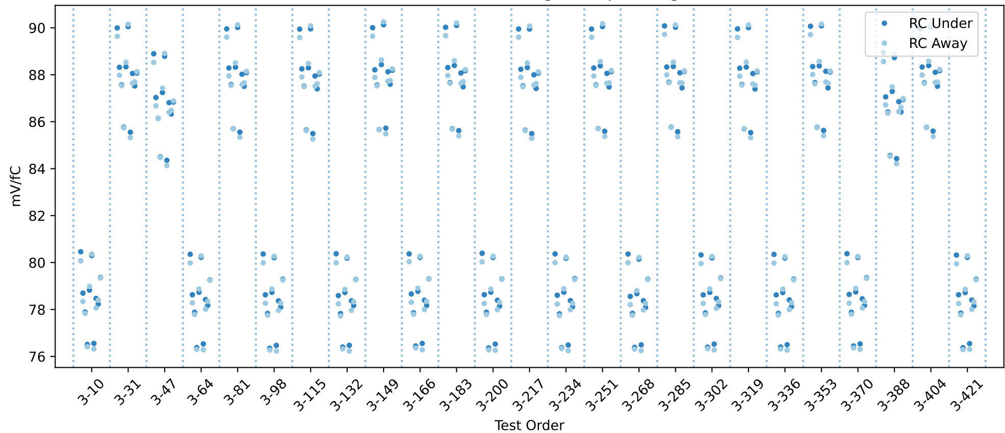
20USBHX2002768 RC gain chip averages
