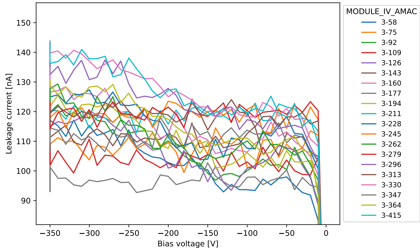
20USBML1236062 fast IV
