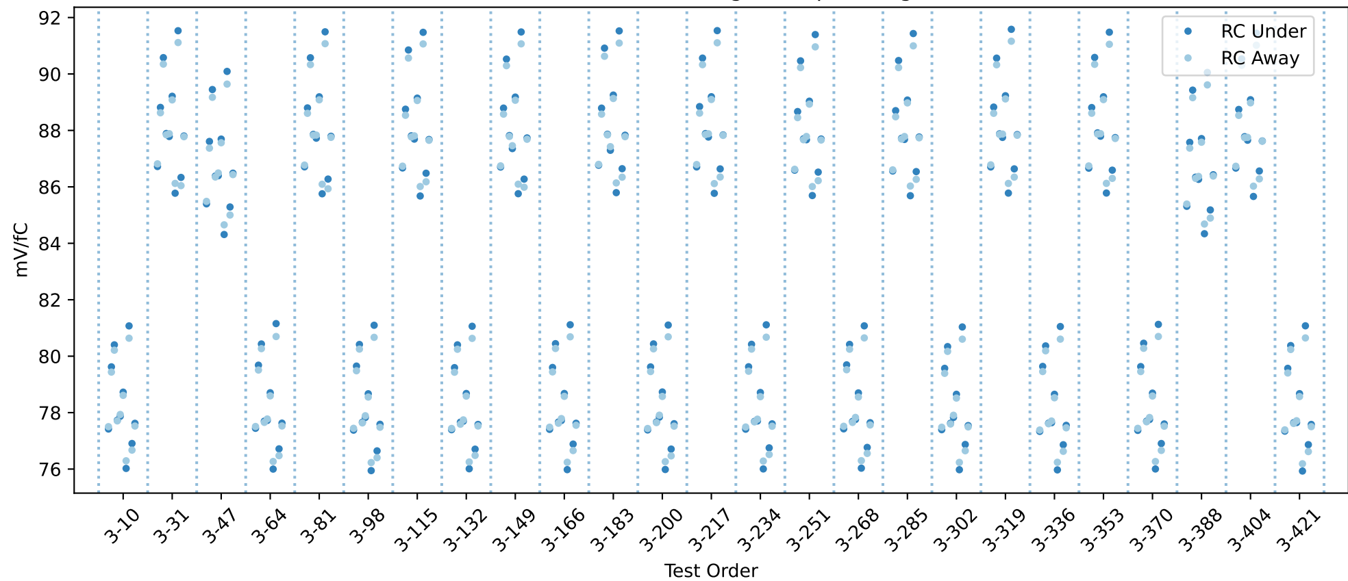
20USBHX2002916 RC gain chip averages
