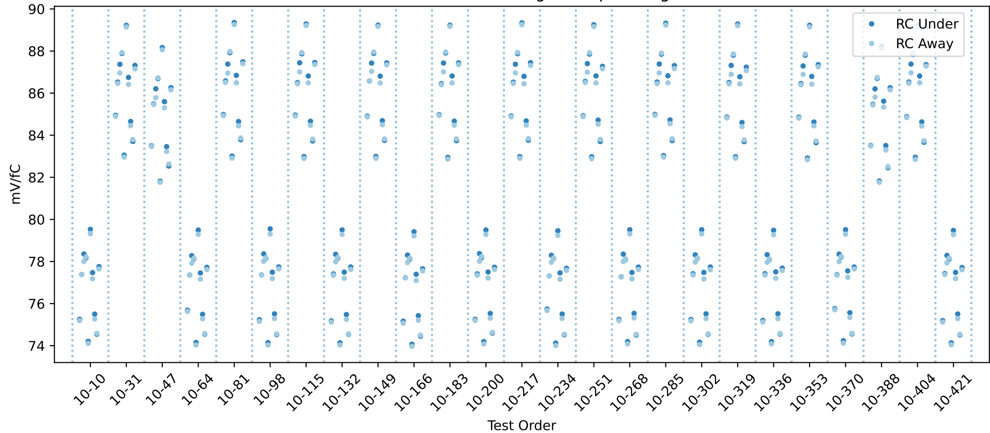
20USBHX2002906 RC gain chip averages
