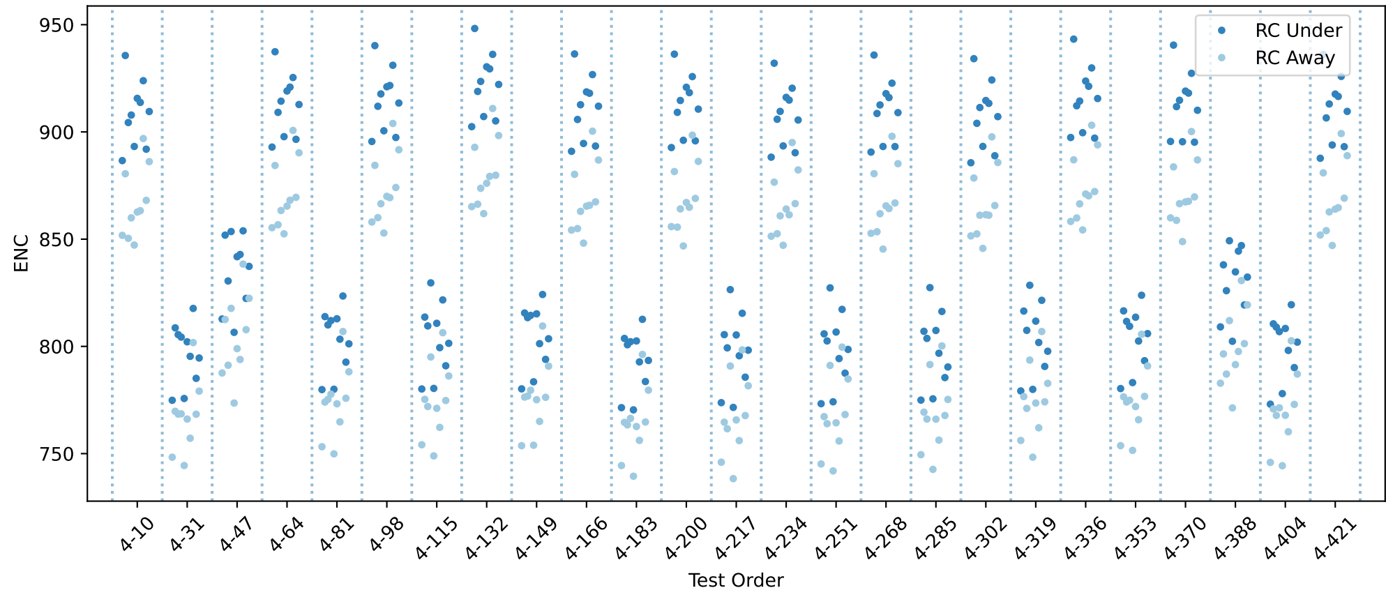
20USBHX2002917 RC innse chip averages
