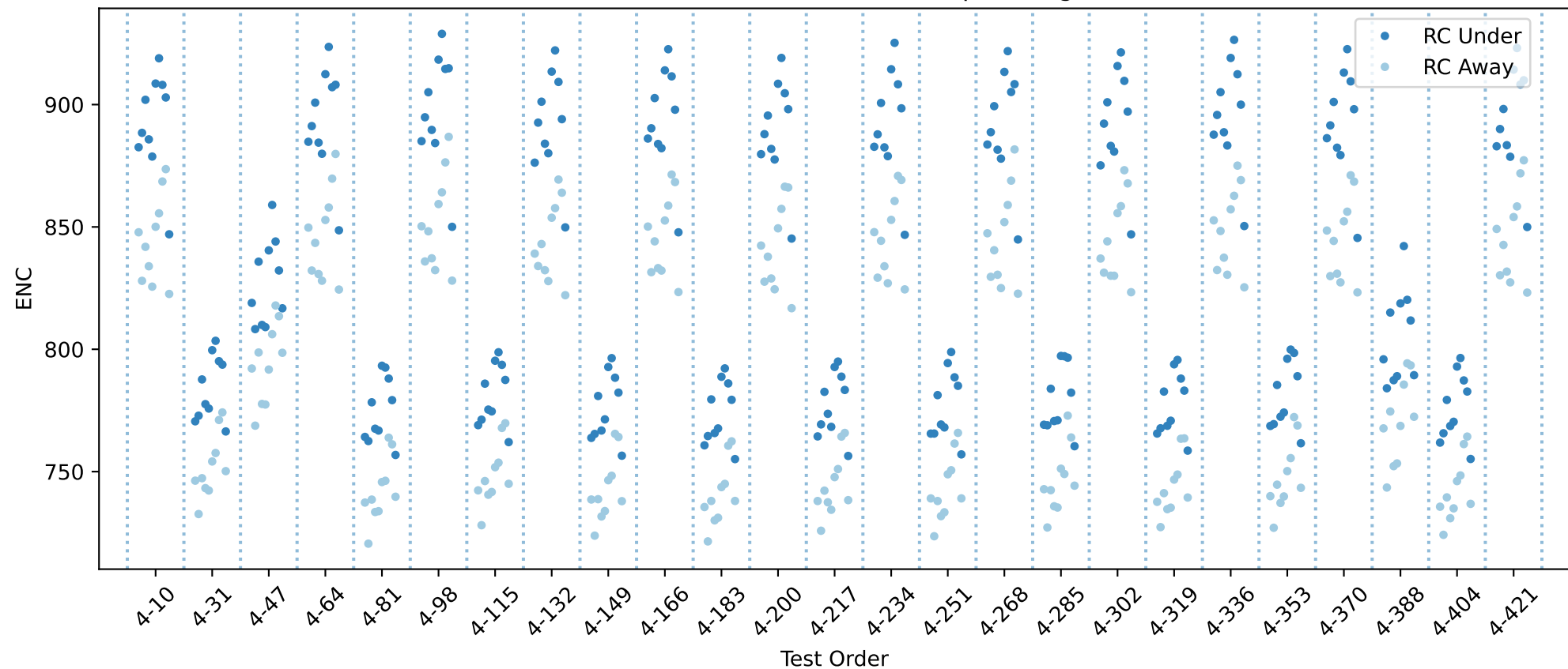
20USBHX2002920 RC innse chip averages
