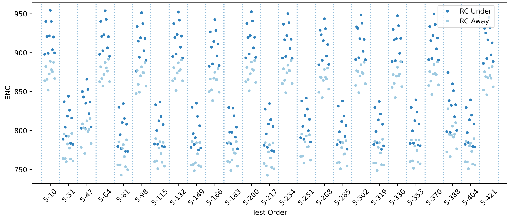
20USBHX2002791 RC innse chip averages
