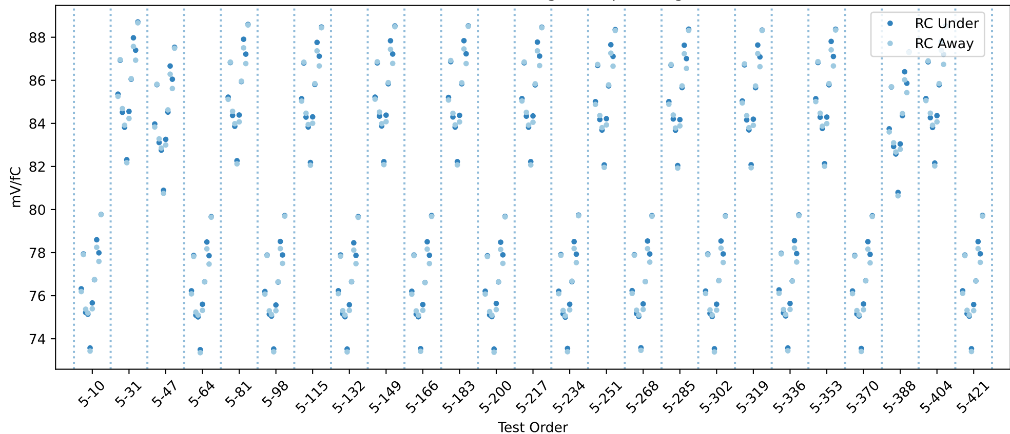
20USBHX2002793 RC gain chip averages
