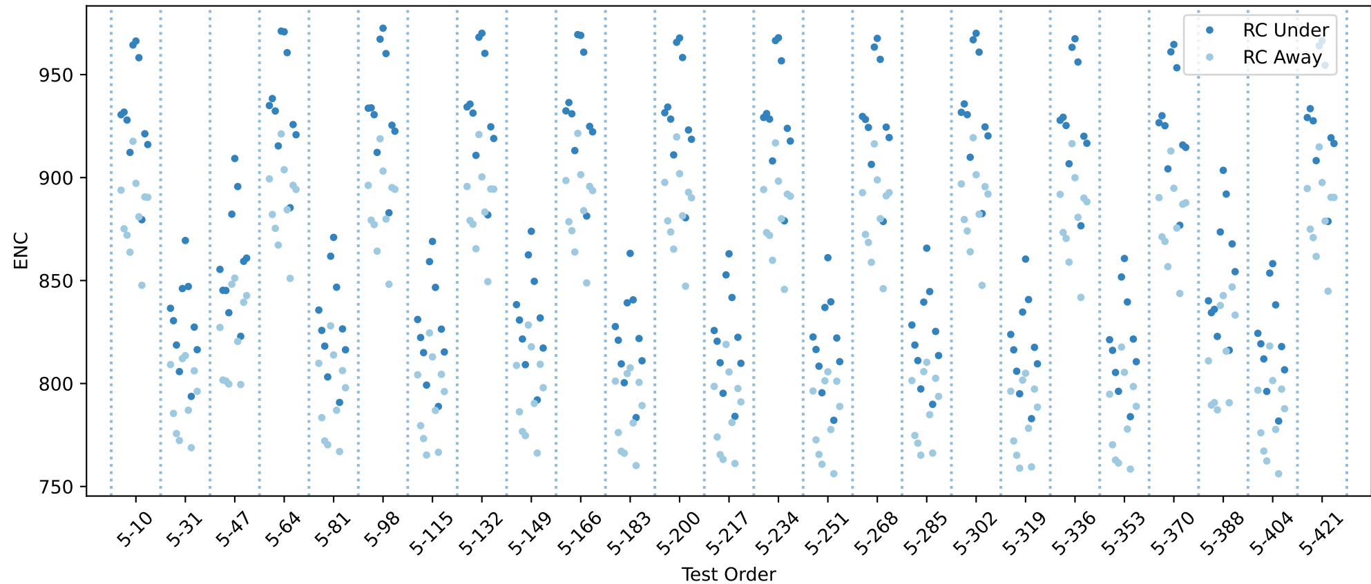
20USBHX2003081 RC innse chip averages
