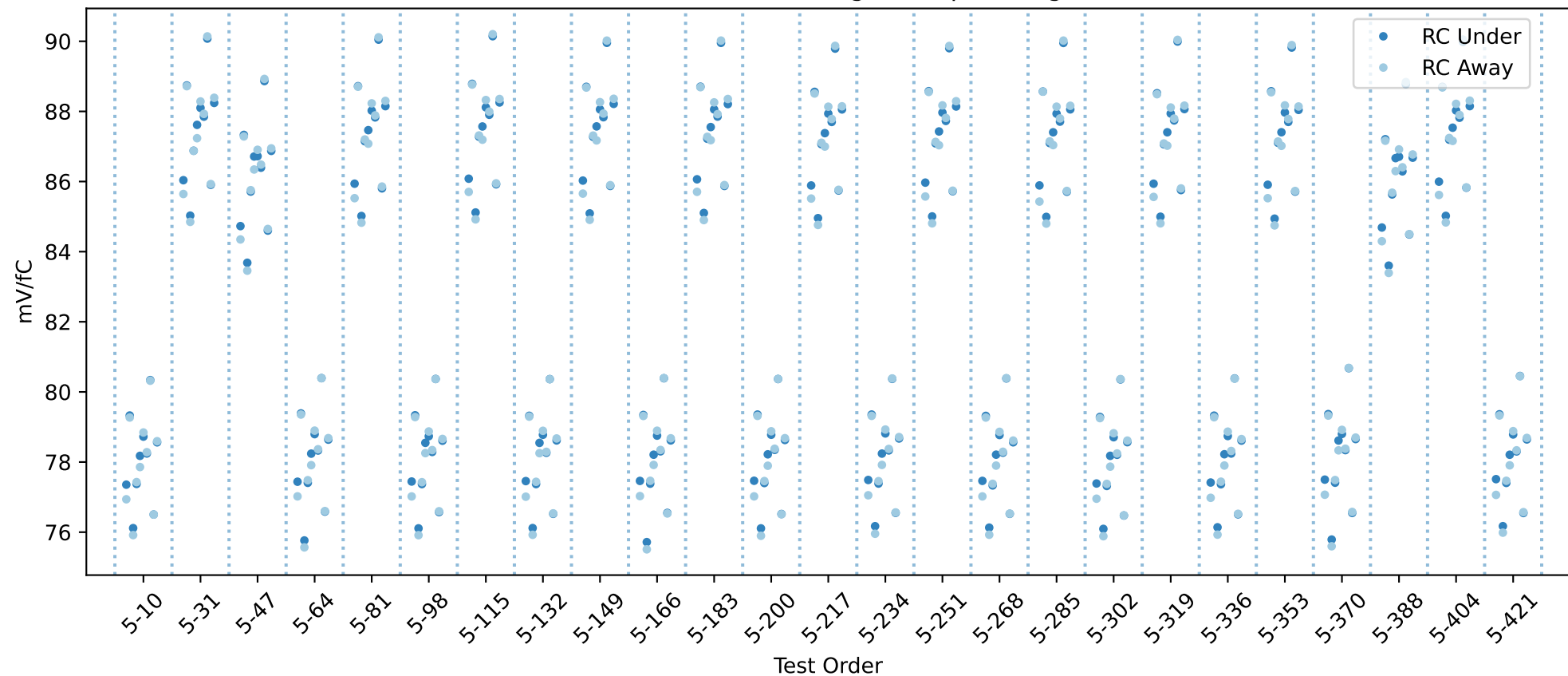
20USBHX2003082 RC gain chip averages
