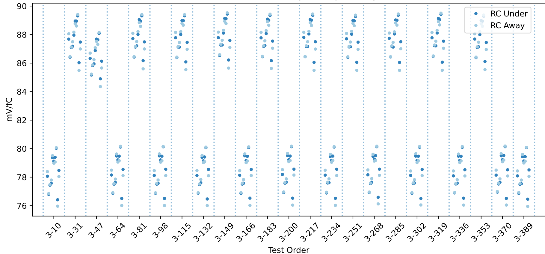
20USBHX2002912 RC gain chip averages
