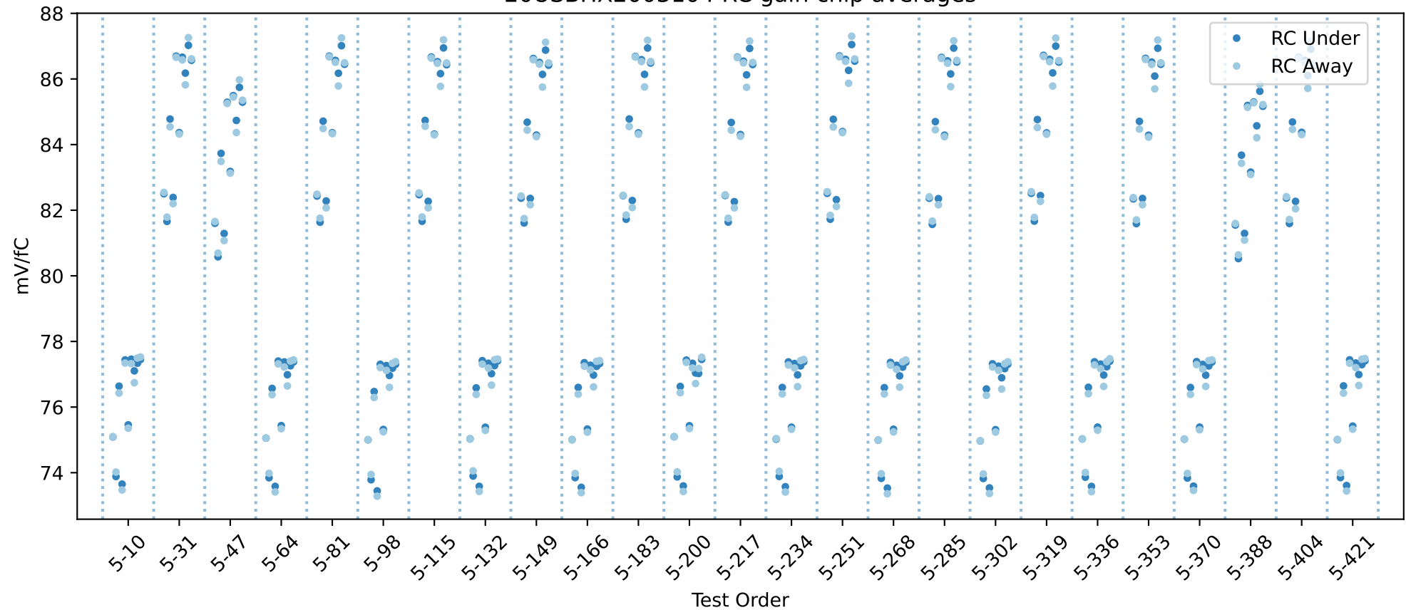
20USBHX2003104 RC gain chip averages
