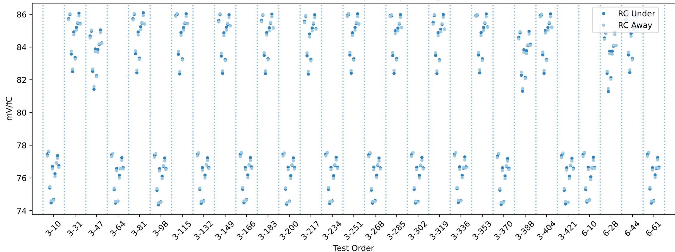
20USBHX2003109 RC gain chip averages
