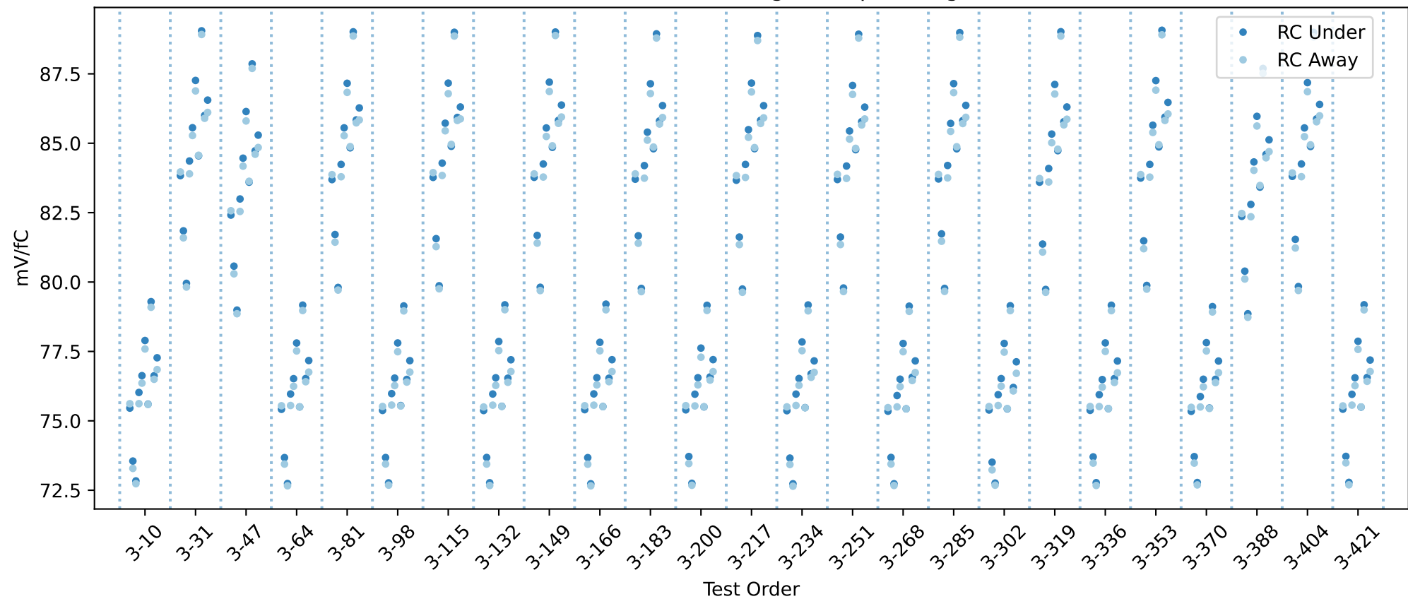
20USBHX2003086 RC gain chip averages
