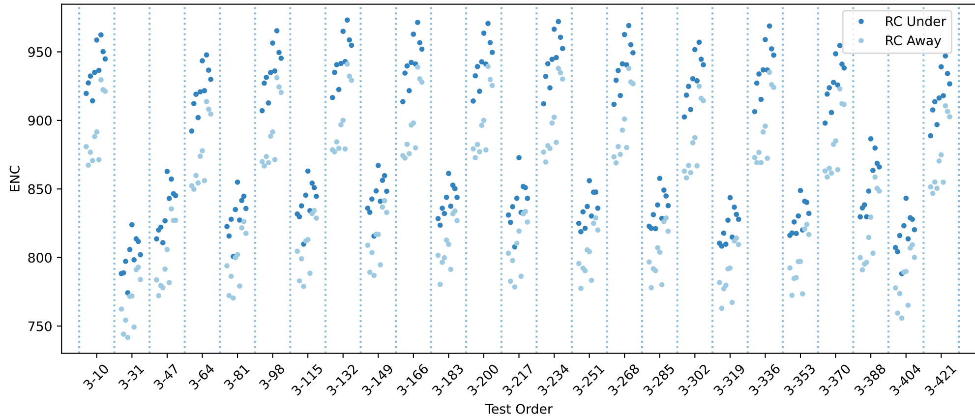
20USBHX2003088 RC innse chip averages
