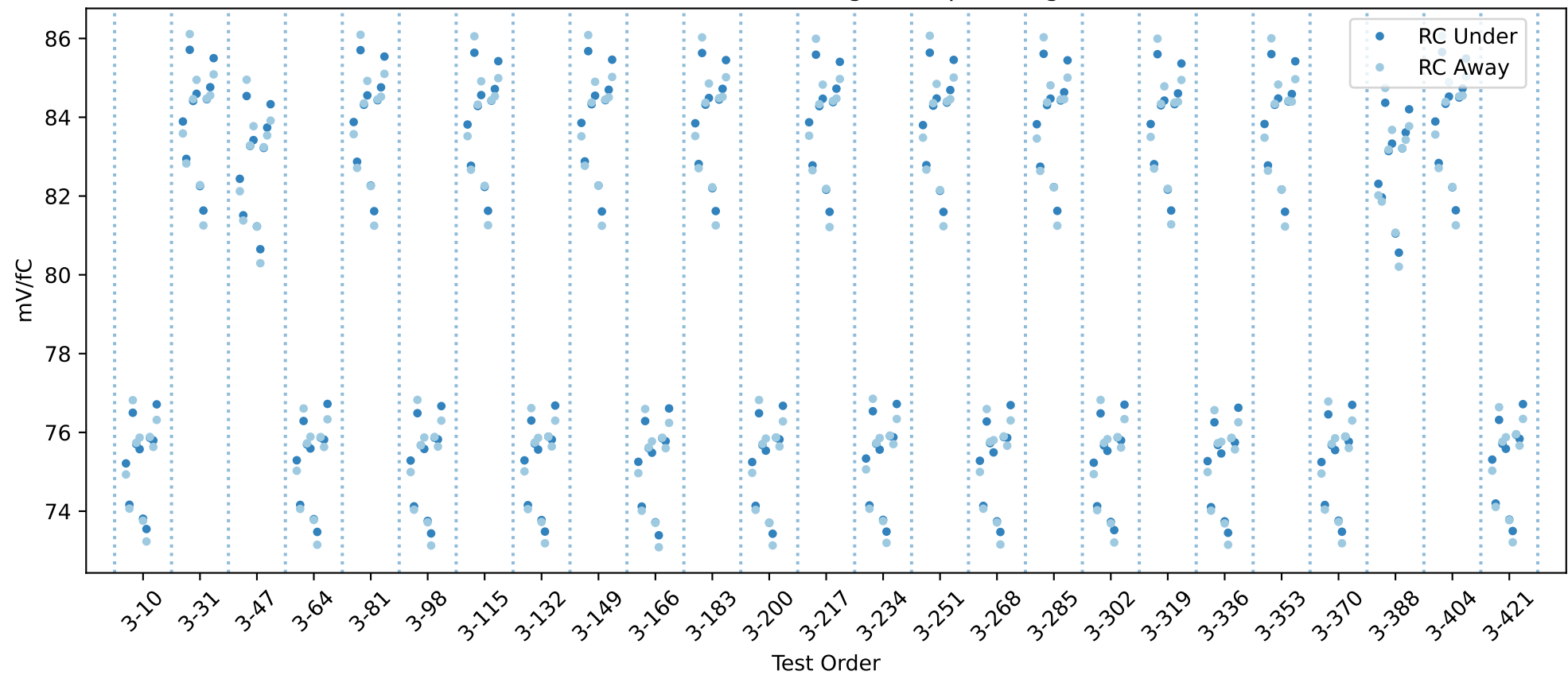
20USBHX2003089 RC gain chip averages
