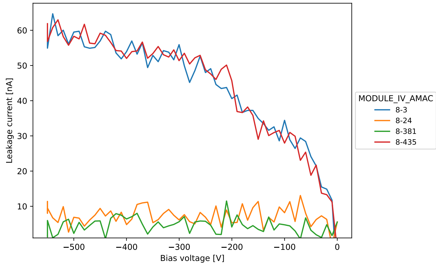
20USBML1236310 standard IV
