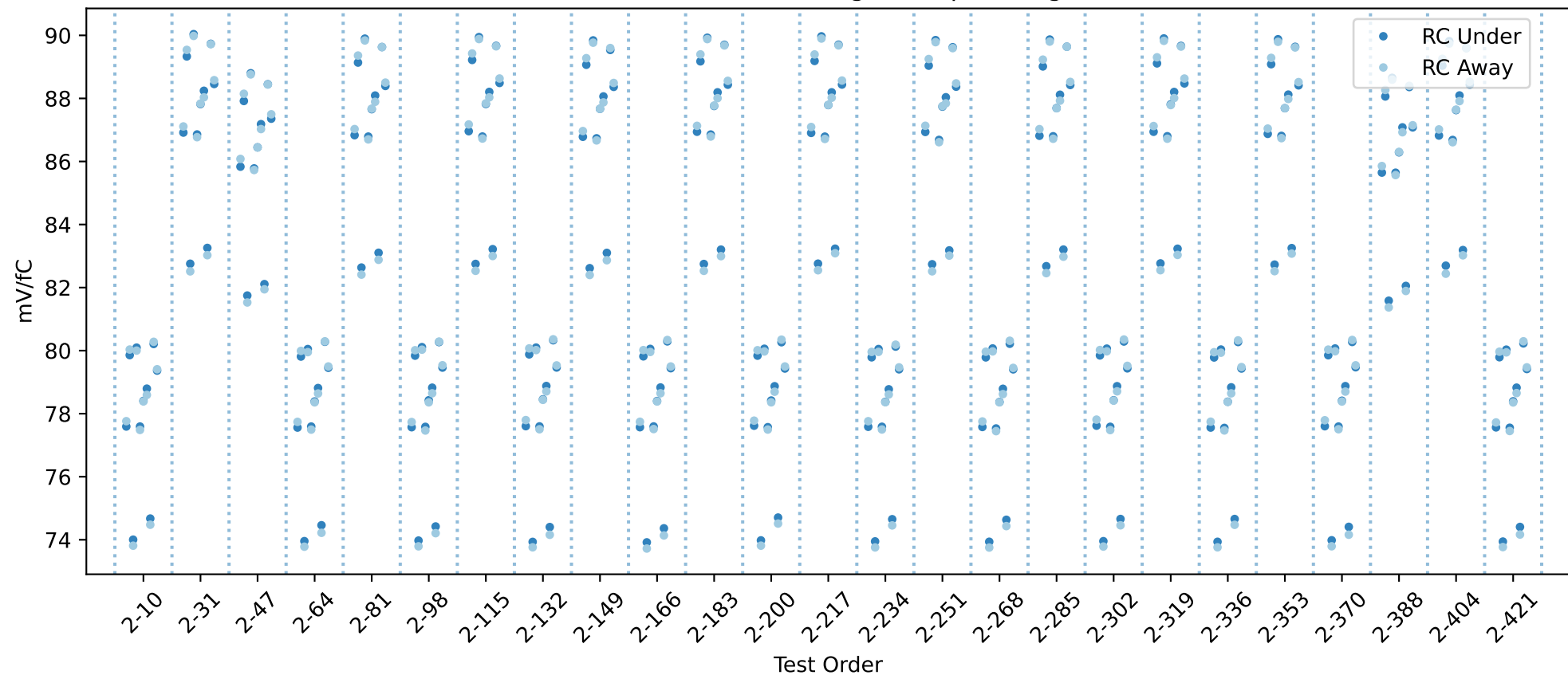
20USBHX2003096 RC gain chip averages
