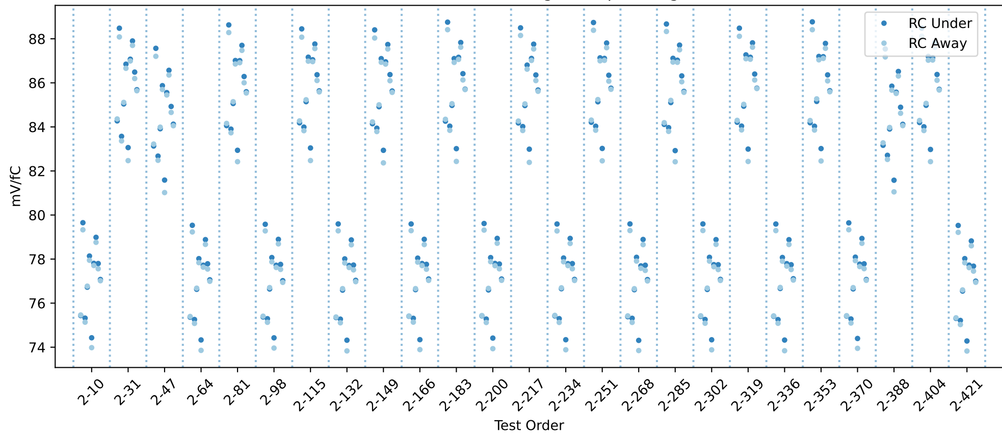
20USBHX2003098 RC gain chip averages
