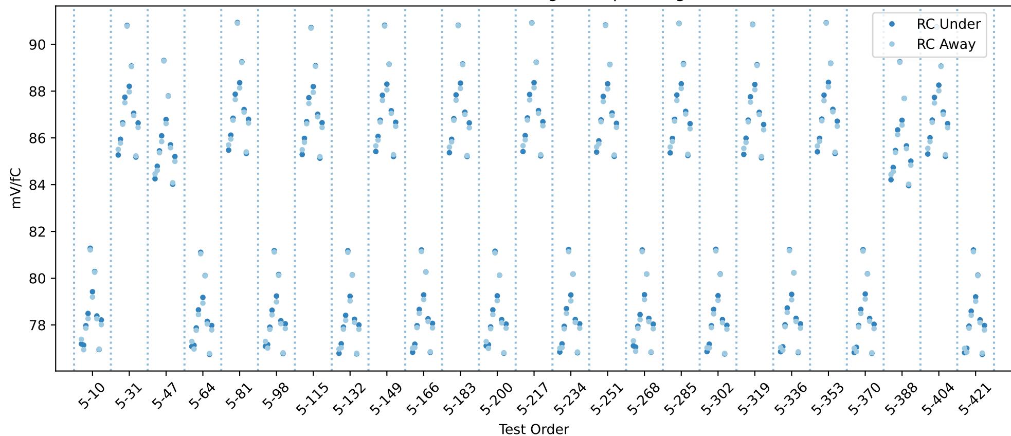
20USBHX2003194 RC gain chip averages
