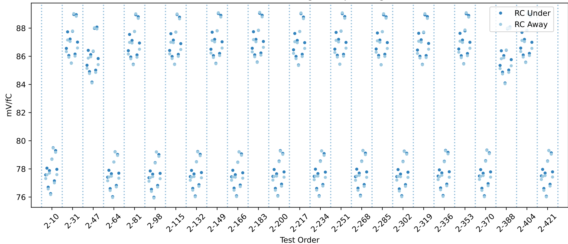
20USBHX2003100 RC gain chip averages
