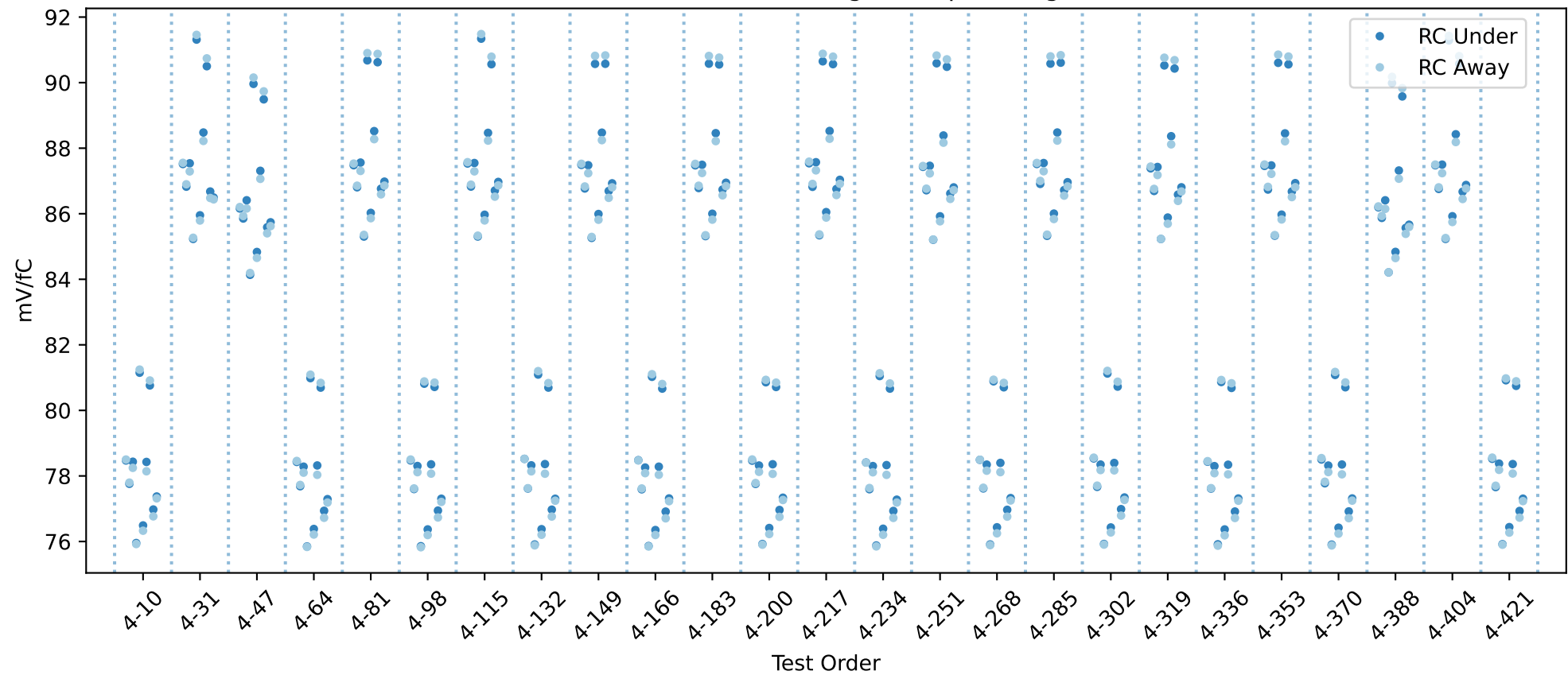
20USBHX2003198 RC gain chip averages
