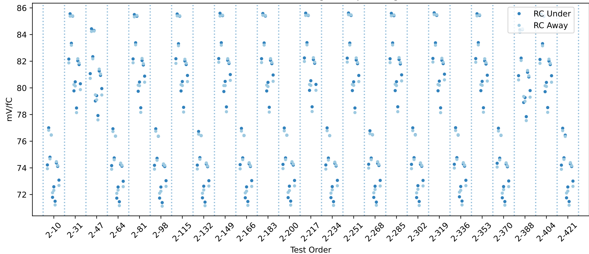
20USBHX2003207 RC gain chip averages
