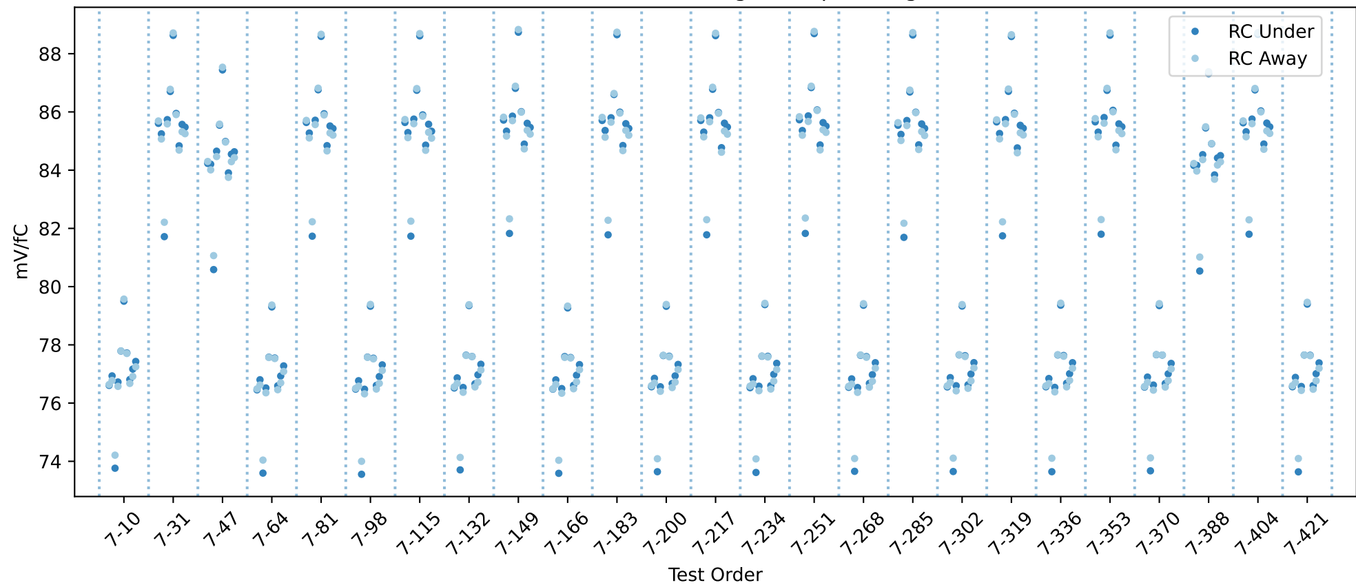
20USBHX2003230 RC gain chip averages
