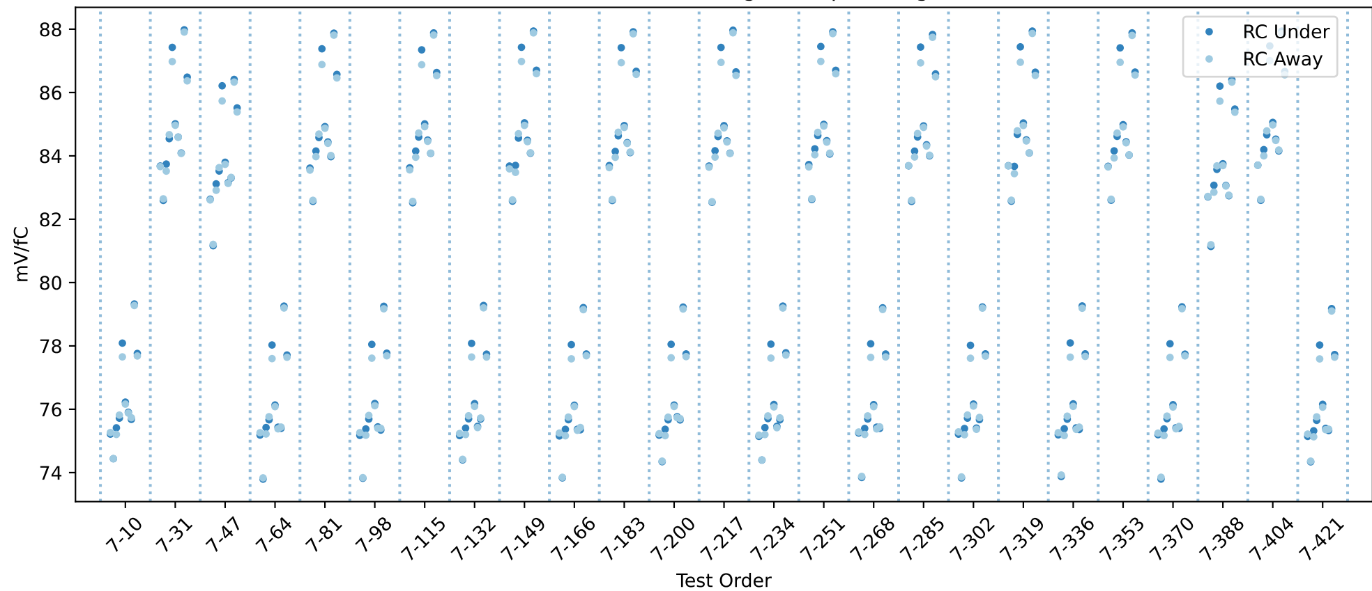
20USBHX2003215 RC gain chip averages
