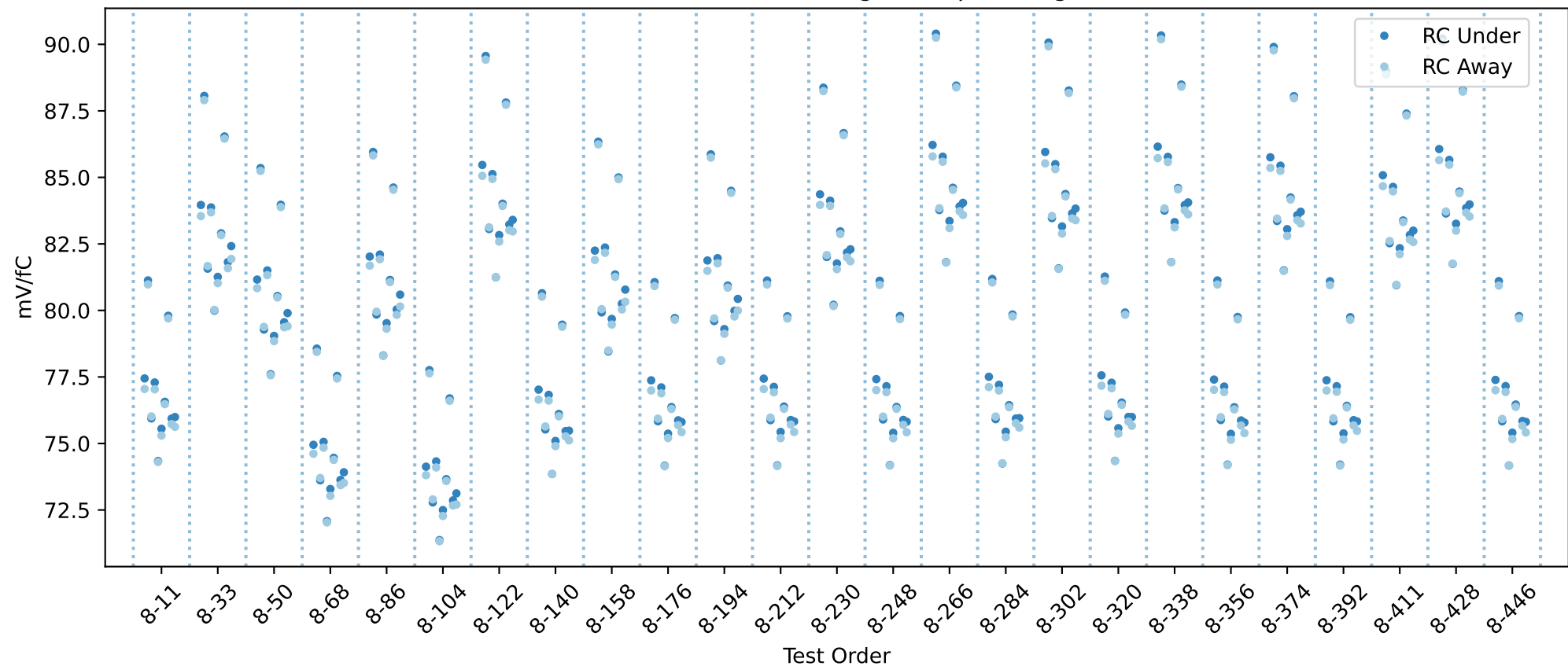
20USBHX2003220 RC gain chip averages
