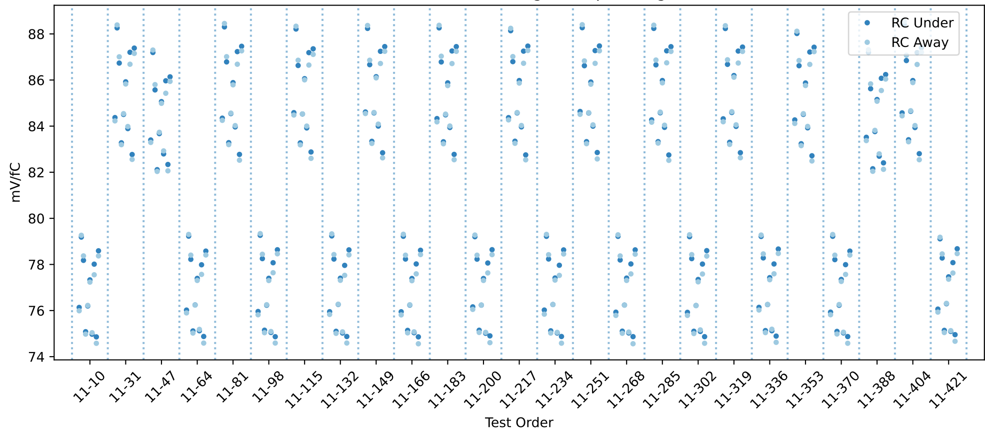
20USBHX2003221 RC gain chip averages
