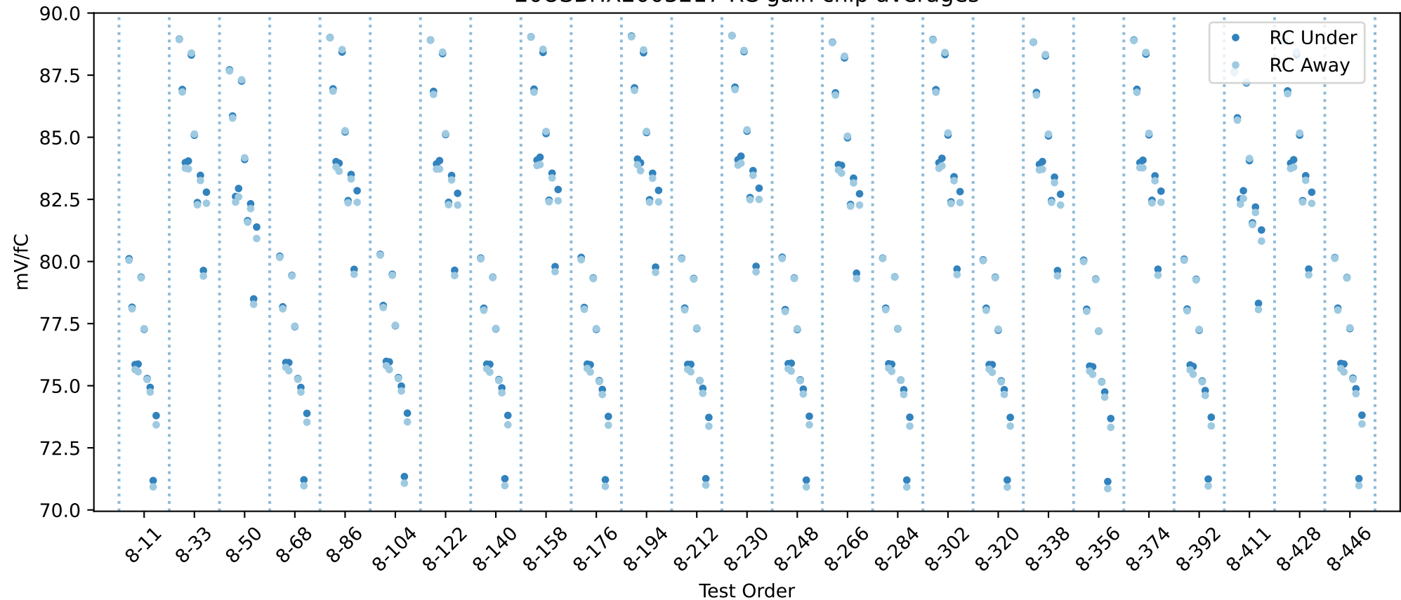
20USBHX2003217 RC gain chip averages
