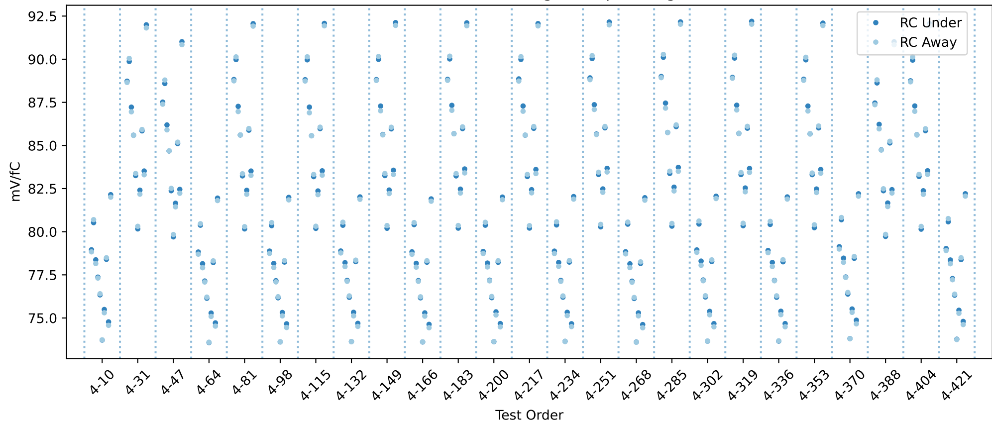
20USBHX2003369 RC gain chip averages
