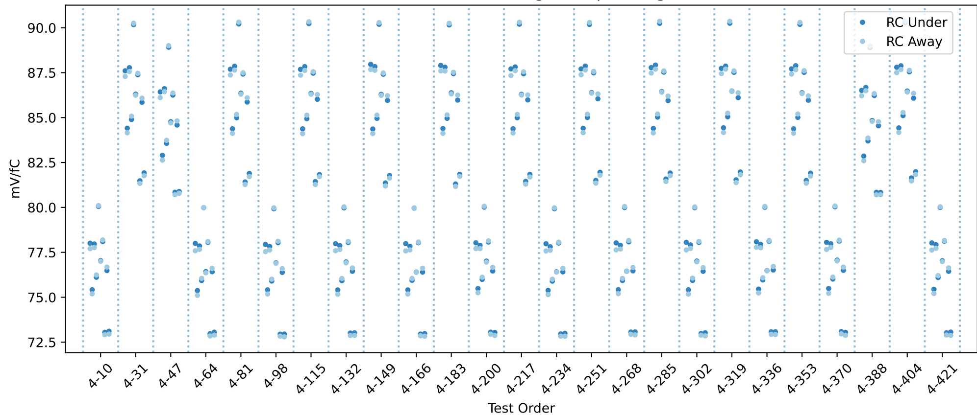
20USBHX2003362 RC gain chip averages
