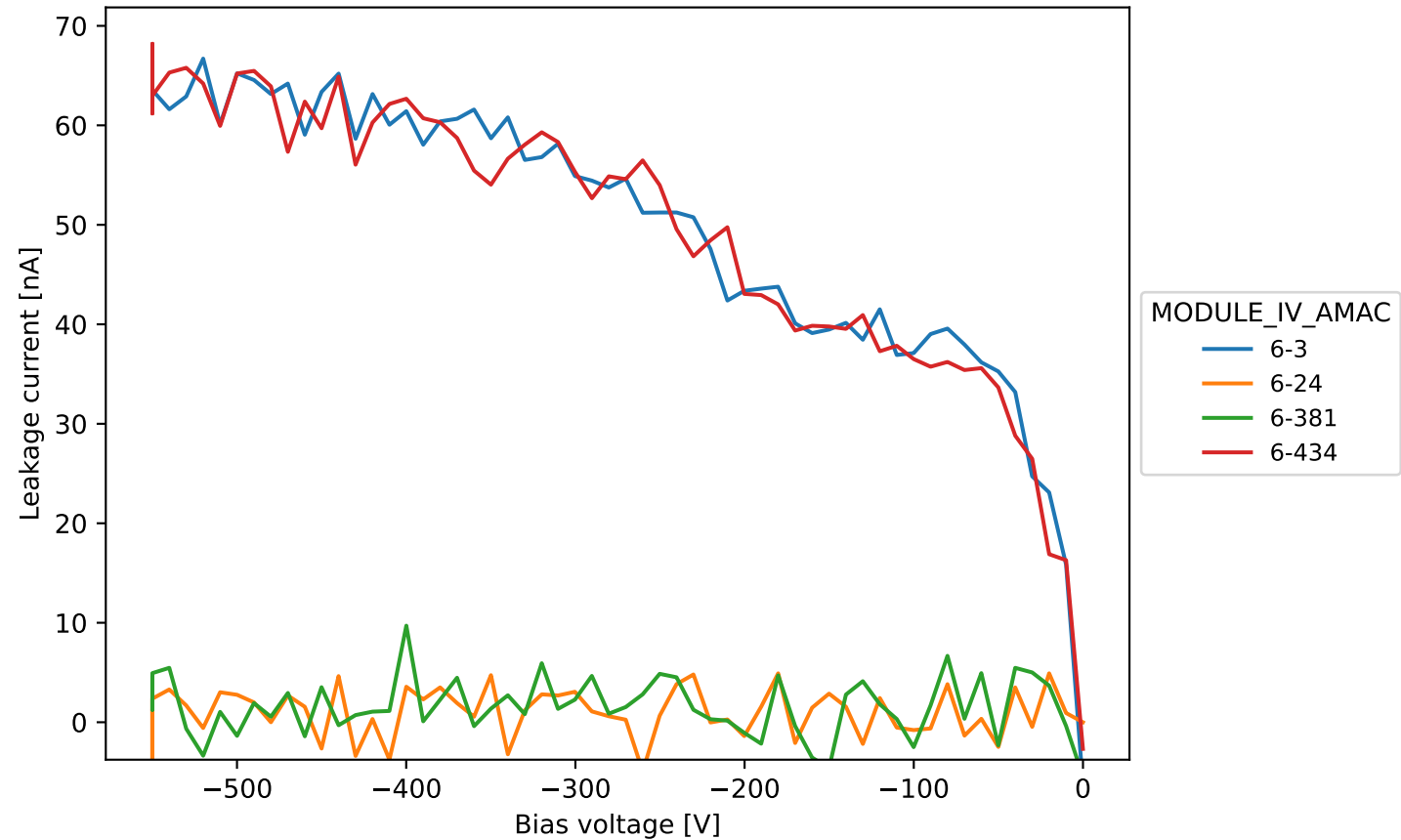
20USBML1236430 standard IV
