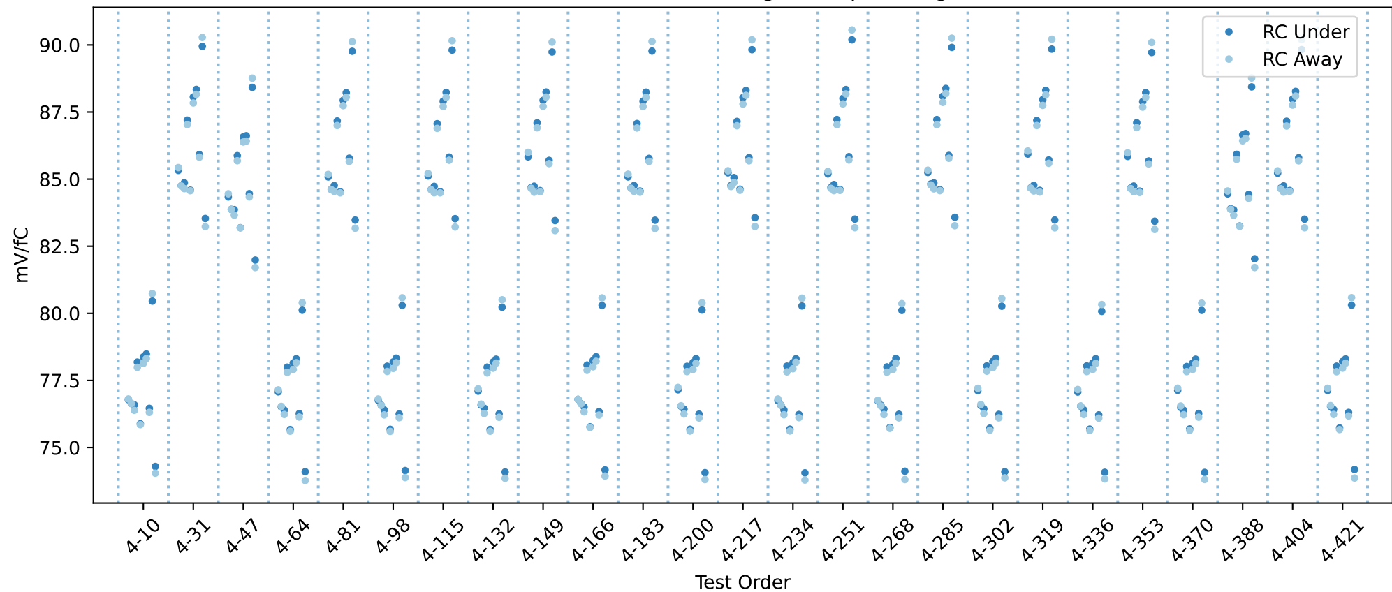
20USBHX2003353 RC gain chip averages
