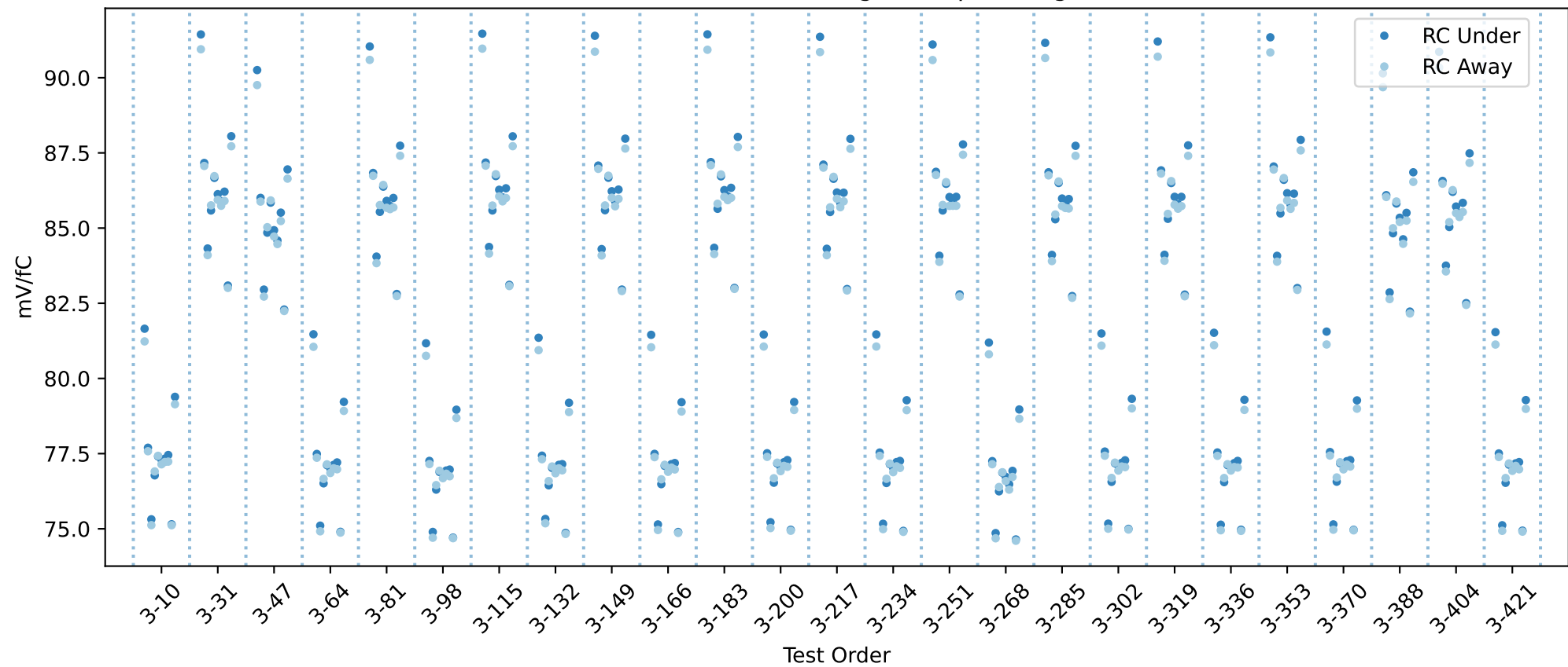
20USBHX2003360 RC gain chip averages
