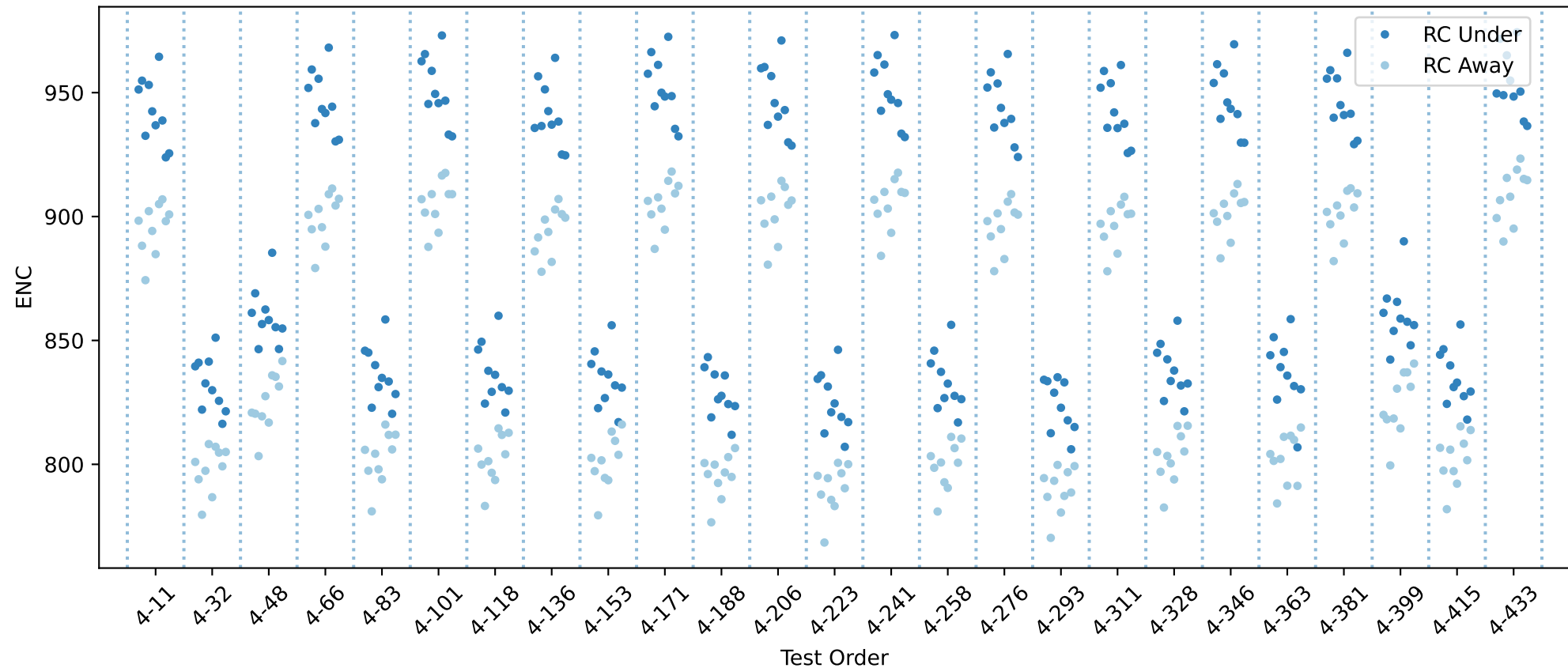
20USBHX2003344 RC innse chip averages
